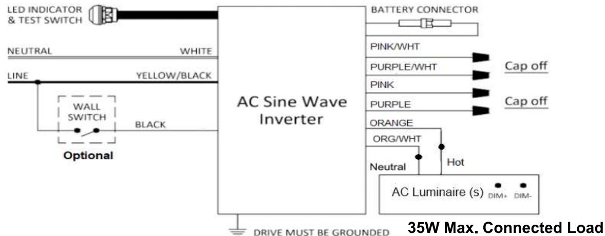
Figure B. Wiring Diagram without 0-10V Dimmer
